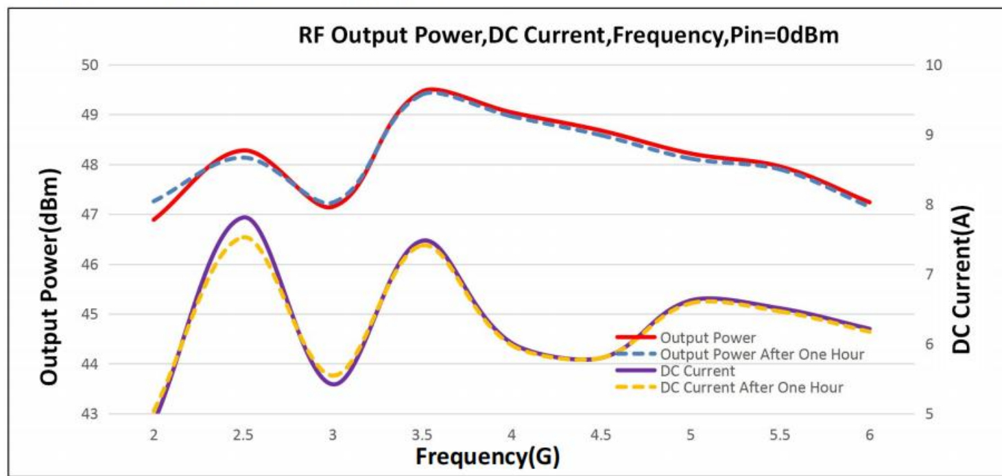
Graph 1: RF Output Power (Low temp. -20\pm 3^{\circ}\text{C} )
