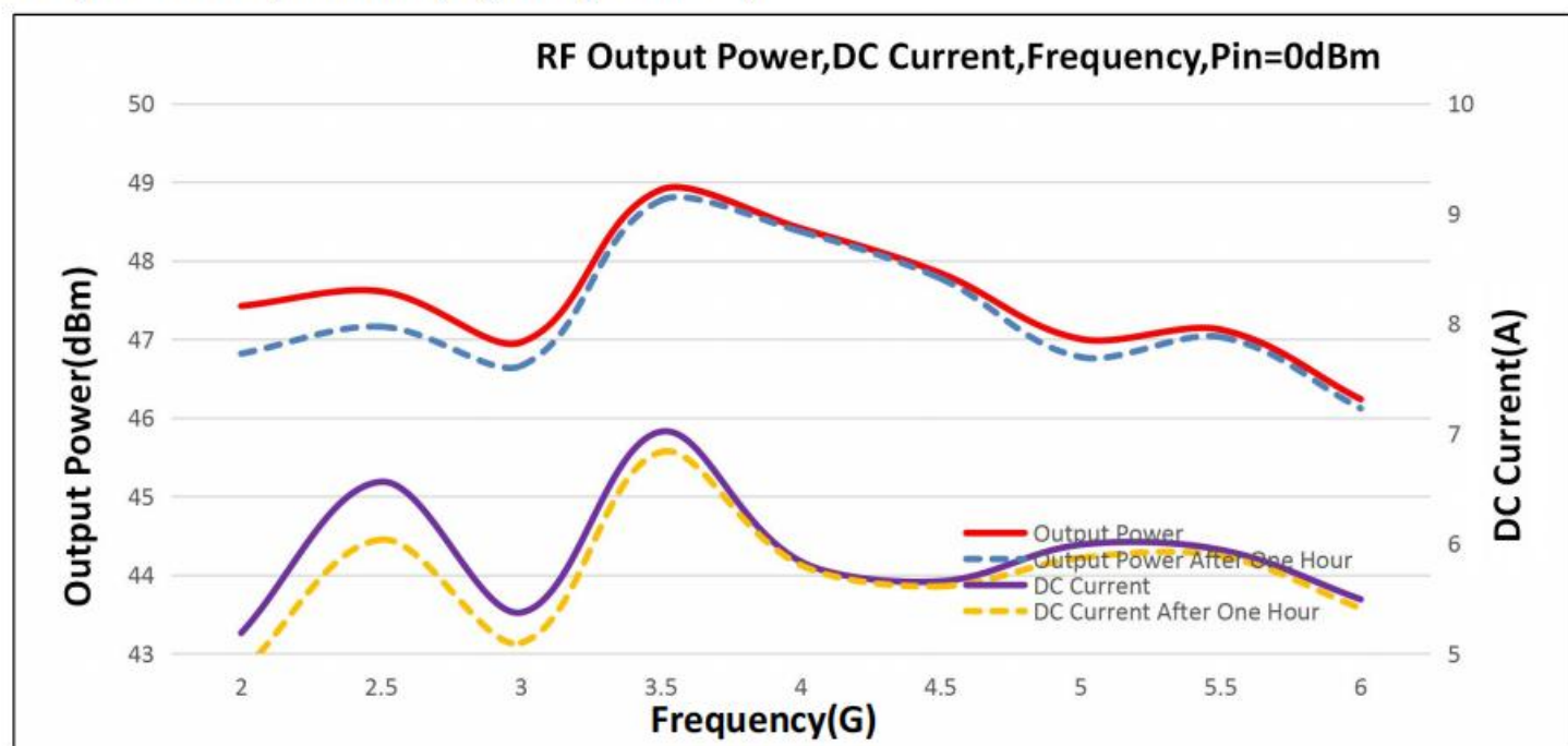
Graph 2: RF Output Power (High temp. +60\pm 3^{\circ}\text{C} )
