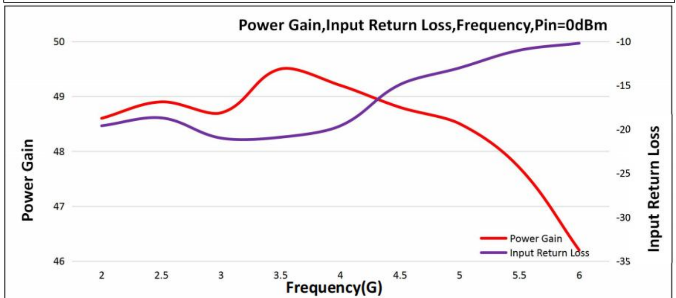
Graph 4: Power Gain, Input Return Loss
